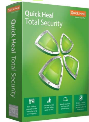
ANTIVIRUS
